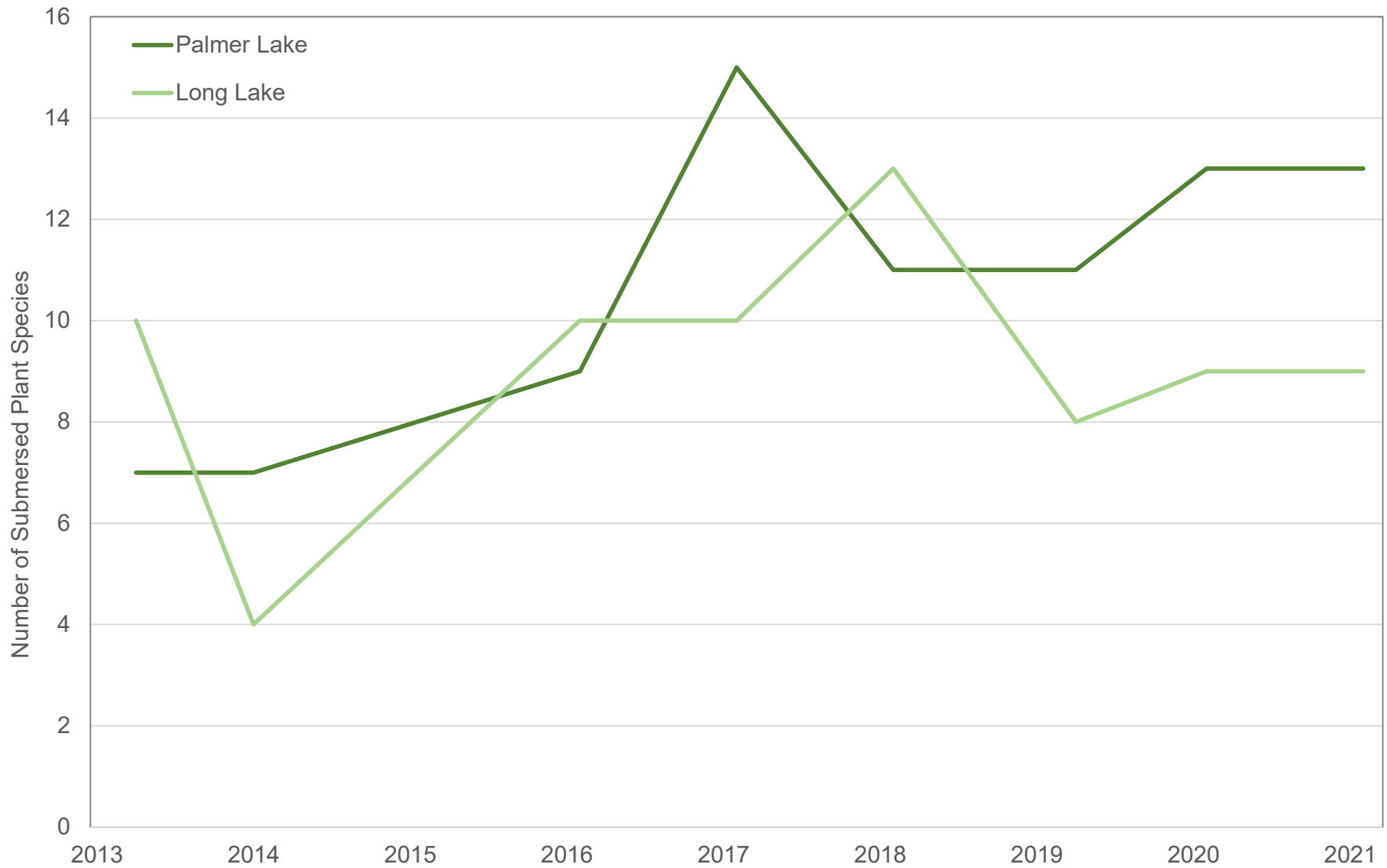
Number of Submersed Plant Species 2013 - 2021
